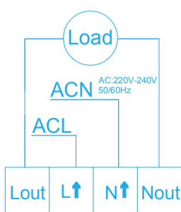
Fig.3 Wiring Diagram
