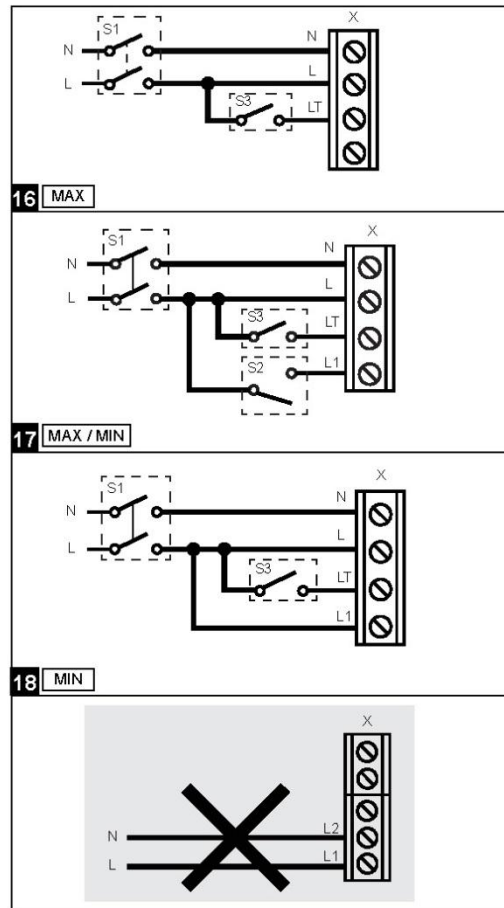
Fig. 3 Wiring Diagram AV100T, AV125T and AV150T
